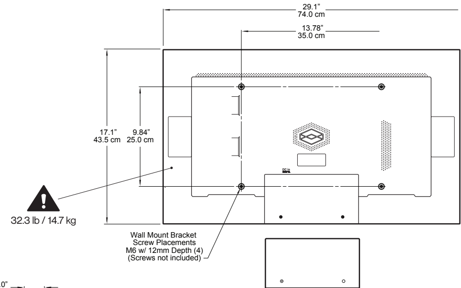
Threaded Inserts (4) for Mounting Figure 1
