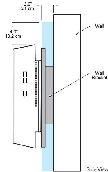
Ventilation - Air Flow Clearances Figure 2
