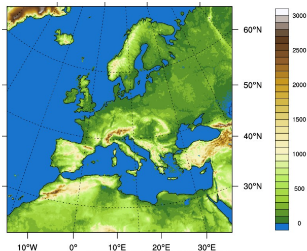
EURO-CORDEX
